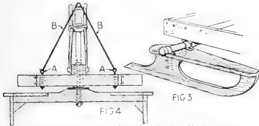
Rear runner and front-bob detail showing the plan of teetering and tilting devices
